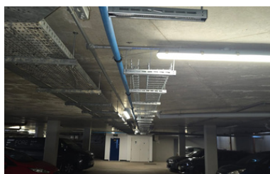
CABLE CONTAINMENT ROUTE
